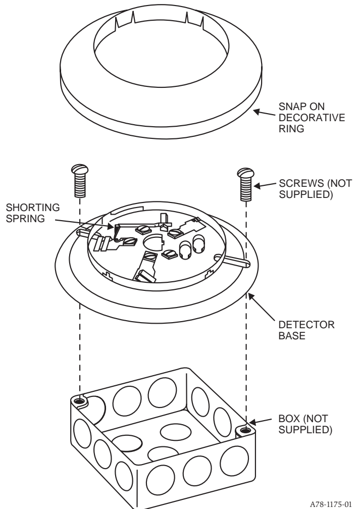
Figure 2. Mounting base to box:
