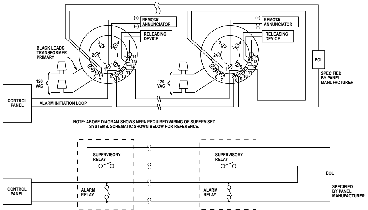
Figure 3. Typical wiring diagram for 120VAC detector systems:
