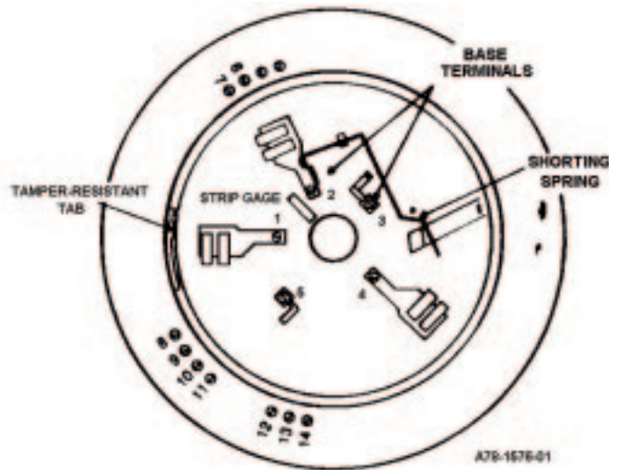
Figure 1. Base terminals:
