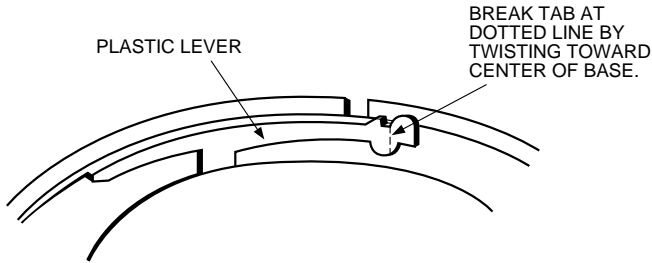
Figure 4A. Activating tamper-resistance feature:
