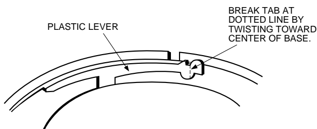
Figure 4A. Activating tamper-resistance feature:
