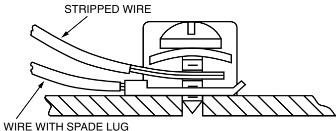
FIGURE 4. CONNECTION TO REMOTE ANNUNCIATOR TERMINAL:
